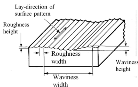
Fig. 2. Surface characteristics (roughness and waviness) excepting surface form deviation
