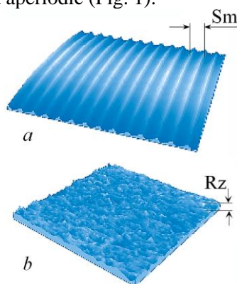
Fig. 1. Periodic (a) and aperiodic (b) profile of a machined surface [4]:
