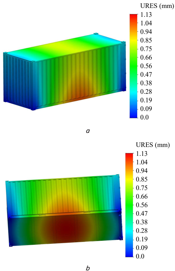
Fig. 10. Movement in the container nodes: a – side view; b – bottom view
