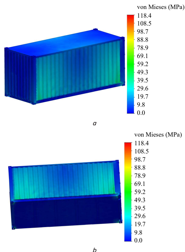
Fig. 9. Stressed state of the container: a – side view; b – bottom view
