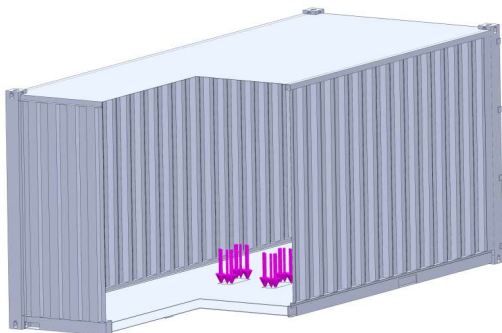
Fig. 12. Container floor loading diagram when moving loading and unloading equipment on the floor
