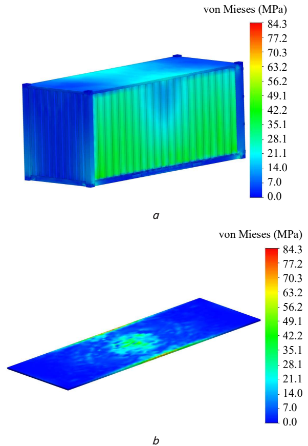
Fig. 13. Stressed state of the container when moving loading and unloading equipment on the floor: a – the container as a whole; b – floor
