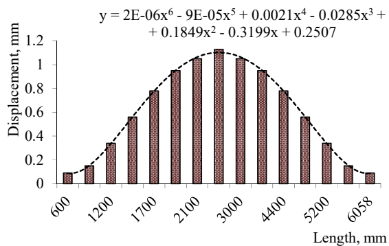
Fig. 11. Distribution of maximum displacements over the lower sheets of the container floor
