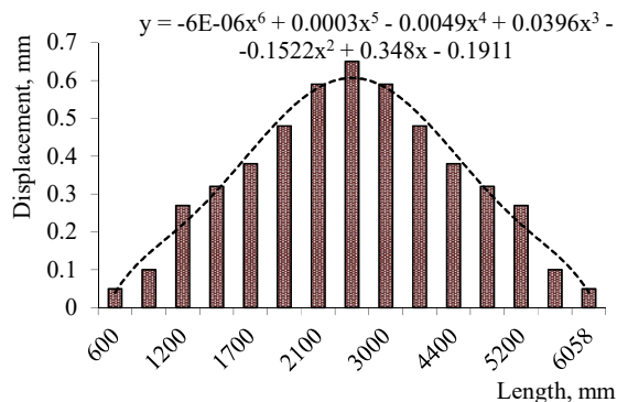
Fig. 15. Distribution of maximum displacements over the lower sheets of the container floor
