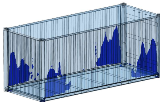
Fig. 8. Most loaded container areas
