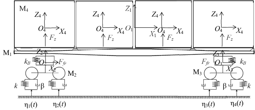
Fig. 4. Calculation diagram of a flat wagon loaded with standard size 1CC containers
