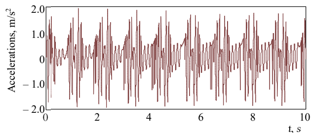
Fig. 5. Accelerations acting on the supporting structure of a flat wagon with containers
