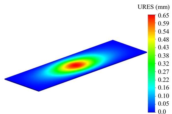
Fig. 14. Movement in the floor of the container when it is loaded by loading and unloading equipment
