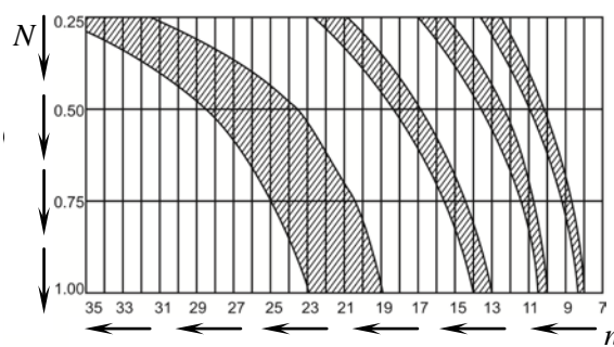
Fig. 2. Complexity of numbers of cavities and protrusions on interrupted wheel and relations of their lengths, forming zones of parametric instability of an elastic system of a plane-grinding machine
