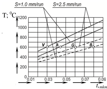
Fig. 8. Dependence of the grinding temperature on the cutting depth when grinding with continuous (continuous lines) and intermittent ( n=12 ; N=0.5 ) (dashed lines) wheels 24A40SM1K1 made of cemented steel 12X2H4A at V_{gem}=10 m/min; V_{kp}=30 m/s
