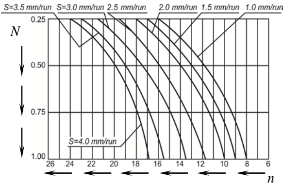
Fig. 3. Curves of equal temperatures separating the non-burning zone from the burner when grinding intermitted wheel 24A40CM1K1 of cemented steel 12X2H4A at the modes: V_{gem}=10 m/min, t=0.075 mm, 1 mm/run \leq S \leq 4 mm/run, V_{kr}=30 m/s
