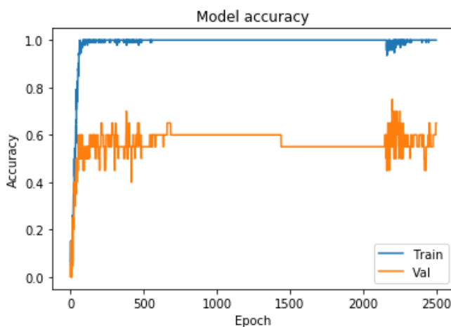
Fig. 9. Diagram of the average accuracy of the CNN model during training (after 2500 iterations) for training and validation sets
