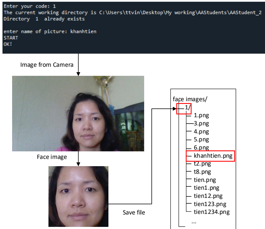
Fig. 8. An example of adding a student's face image from a camera to the dataset
