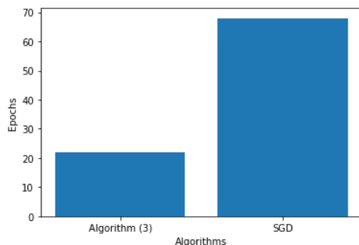
Fig. 5. Bar graph of performance differences between algorithm (3) and SGD
