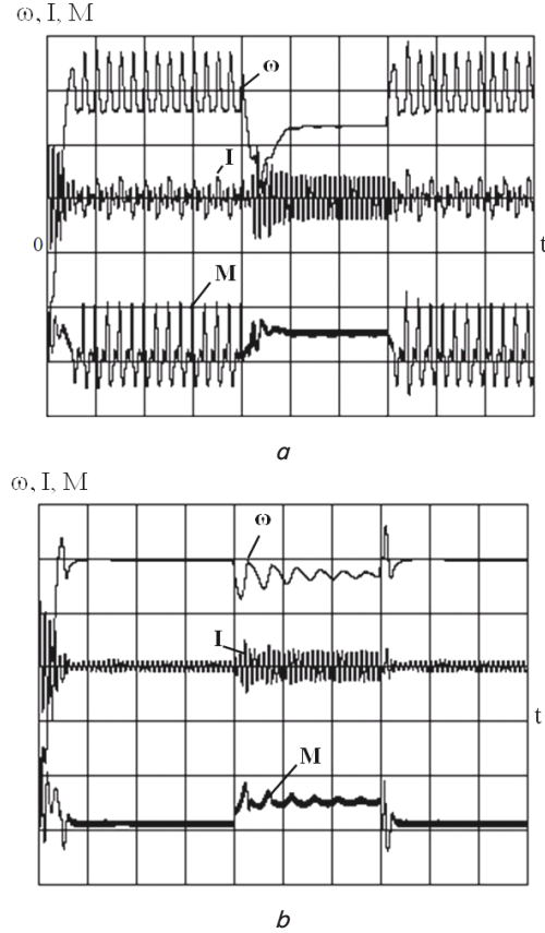
Fig. 12. Waveforms of the processes of switching and load acceptance and shedding of the motor 4A100L4, 4 kW, J_{\text{sum}} = 1.1J_{\text{IM}} : a – controlling action \alpha = 70 el. degrees; b – controlling action U_1 = 0.85U_n . The constants scale: m_t = 0.2 \text{ c/div.} ; m_m = 2 \text{ Mn/div.} ; m_\omega = 0.2\omega_0/\text{div}
