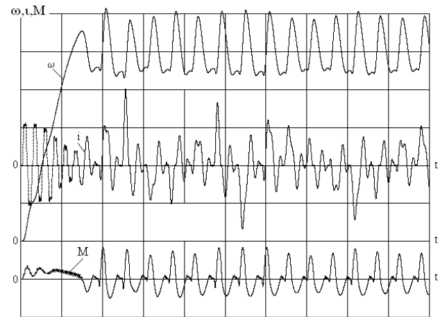
Fig. 11. Waveform of a transient process of switching and an oscillations mode of ED 4A100M4, 3 kW, with switching angle \alpha=83 el. degrees; M_s=0.01M_n ; J=1.05J_{IM} for the case of SPPC-3. Scale: m_i=25A/div. ; m_m=4M_n/div. ; m_{\omega}=0.2\omega_0/div , m_t=0,08s/div
