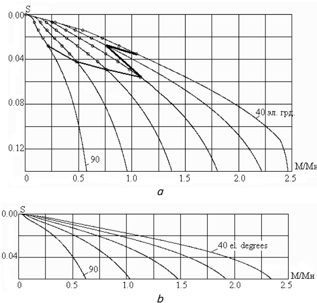
Fig. 8. Families of mechanical characteristics with certain areas of unstable performance for motors: a – 4A200L4; b – 4A355S4
