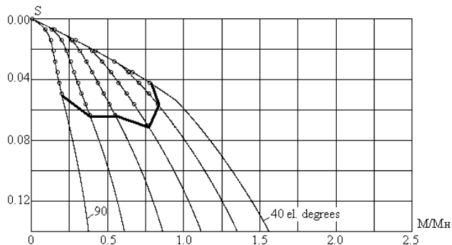
Fig. 9. Mechanical parameters with the indication of the area of unstable performance of TVC-IM with the engine 4A100L4, aggregated inertia torque J_\Sigma=2J_{IM}
