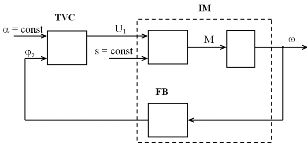
Fig. 3. Estimated structural scheme of an open-loop system of ED TVC-IM
