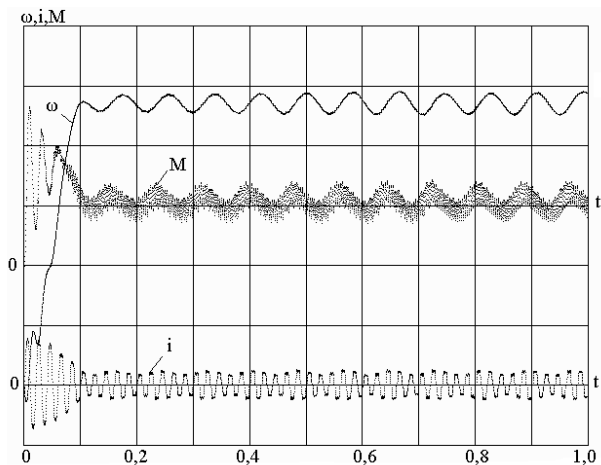
Fig. 1. Charts of the change of velocity \omega , torque M and the stator current i of IM 4A80B4 in a “small” oscillations mode; \alpha=50 el. degrees, M_s=1.1 M_n , J_\Sigma=J_{IM} . Scale: m_i=4I_n/div. ; m_m=1M_n/div. ; m_\omega=0.2\omega_0/div
