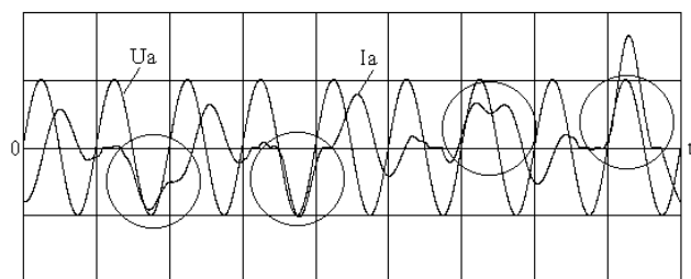
Fig. 10. Waveforms of the phase current of induction motor 4A100M4, 3 kW, in an oscillations mode for the case of SPPC-3 with switching angle \alpha=83 el. degrees; M_s=0.01M_n ; J=1.05J_{IM}
