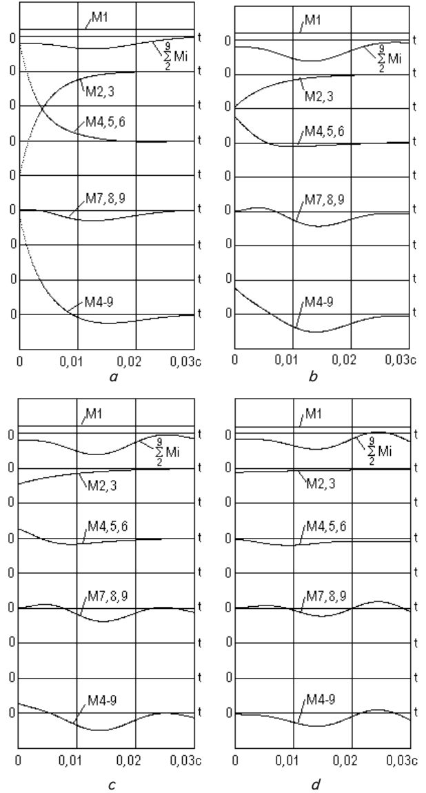
Fig. 5. Charts of equivalent components of electric magnetic torque of IM at switching with zero IEMC at continuous slip s=s_n . The scale of torques 5M_n/\text{div} : a – 4A80A6; 0.75 kW; b – 4A100L4; 4 kW; c – 4A132M4; 11kW; d – 4A355S4, 250 kW
