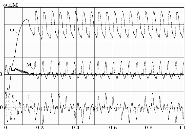
Fig. 2. Charts of the change of velocity \omega , torque M and the stator current i of IM 4A80B4 in a “large” oscillations mode; \alpha=70 el. degrees, M_s=0.5 M_n , J_\Sigma=1.5J_{IM} . Scale: m_i=2.5I_n/div. ; m_m=4M_n/div. ; m_\omega=0.2\omega_0/div
