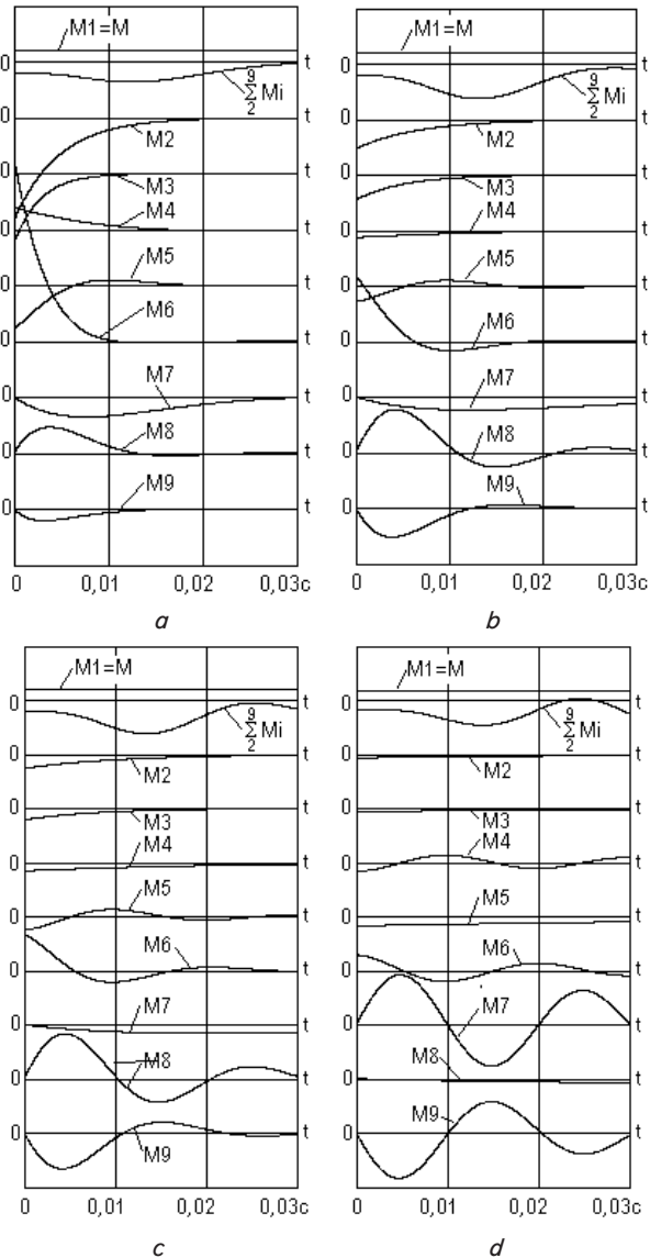
Fig. 4. Charts of the components of electric magnetic torque of IM when switching with zero IEMC during constant slip s=s_n . The scale of the torques 5M_n/\text{div} : a – 4A80A6; 0.75 kW; b – 4A100L4; 4 kW; c – 4A132M4; 11 kW; d – 4A355S4, 250 kW
