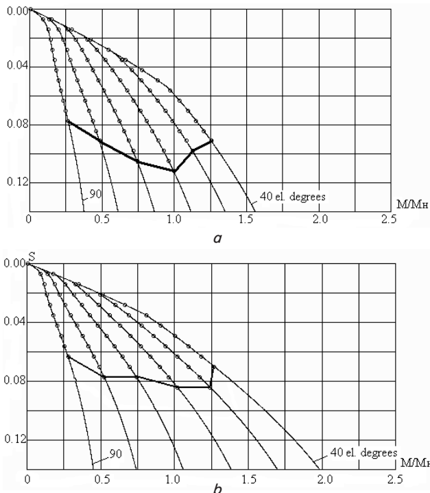
Fig. 7. Families of mechanical characteristics with certain areas of unstable performance for motors: a – 4A100L4; b – 4A132M4
