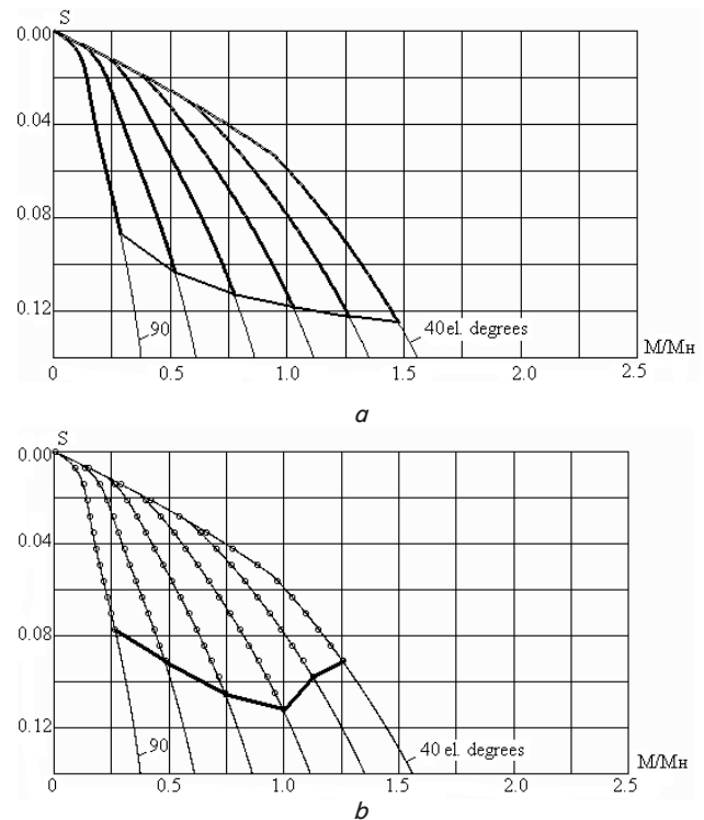
Fig. 6. Families of mechanical characteristics with certain areas of unstable performance by the computational analytical method (a) and by using mathematical and physical IM models of ED TVC-IM (b) for the motor 4A100L4
