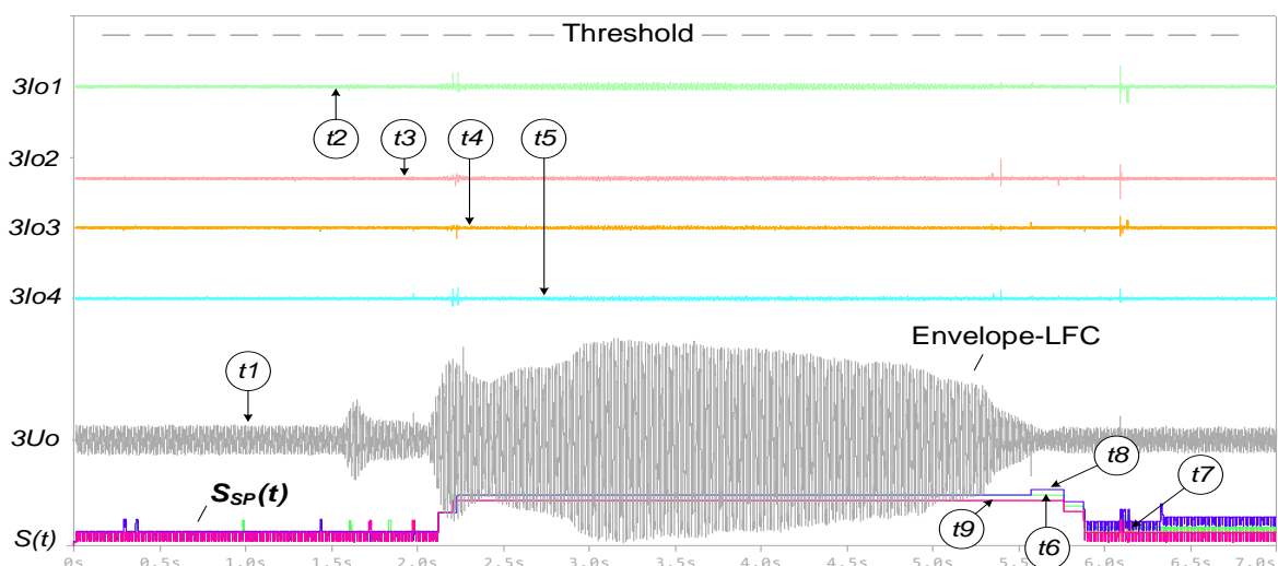
Fig. 9. Modelling of SN in real time SN simulation for 4 ZN sections SN “Neutral offset” t1 - 3U_0 ; t2-5 - signals 3I_0 for Z1-Z4 ; t6-9 - sense signals S(t) for Z1-Z4
