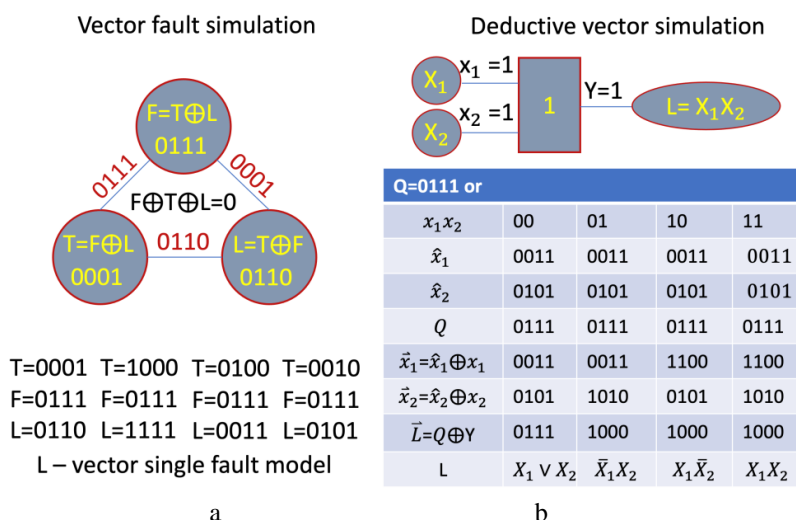
Fig. 3. Deductive-vector or-logic modeling: a – model of single faults; b – procedures for the synthesis of deductive formulas Source: compiled by the author
