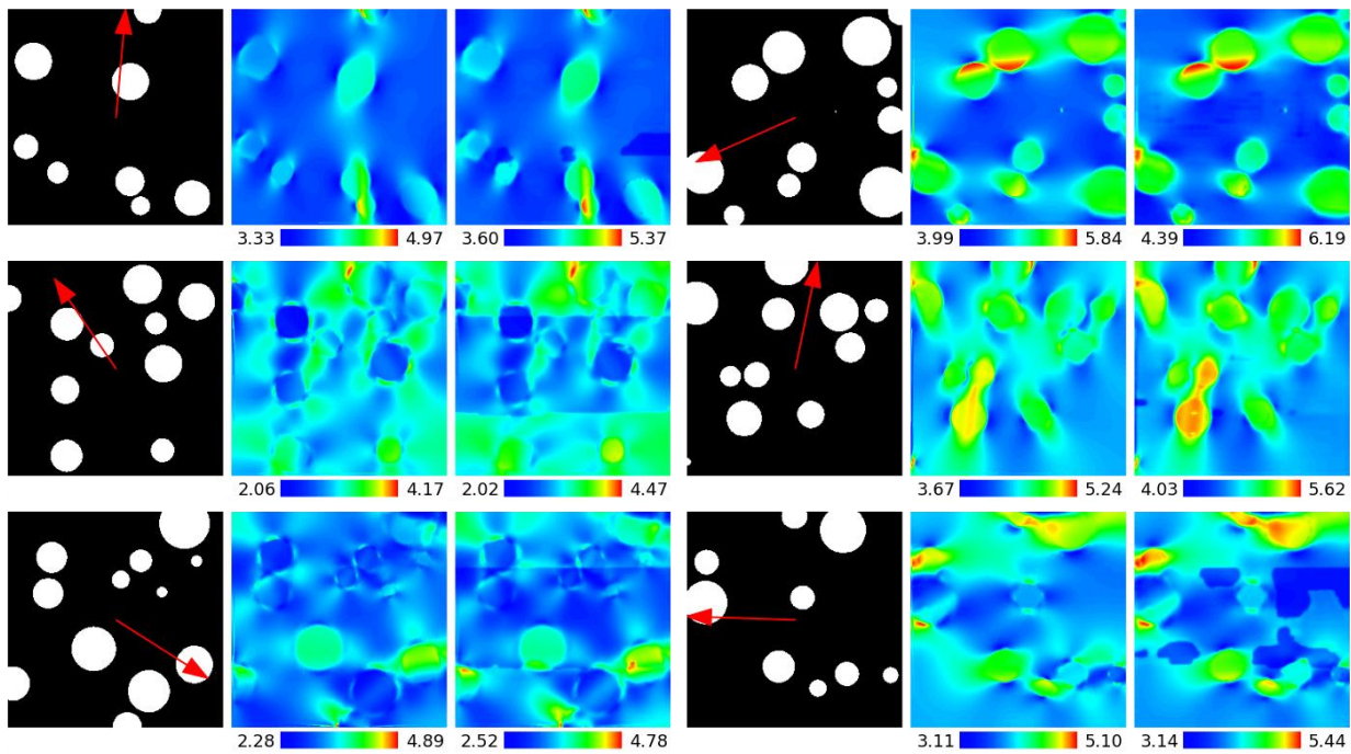
Fig. 17. Sample geometry, MCE solution, and surrogate model output. The test sample, GPa .
