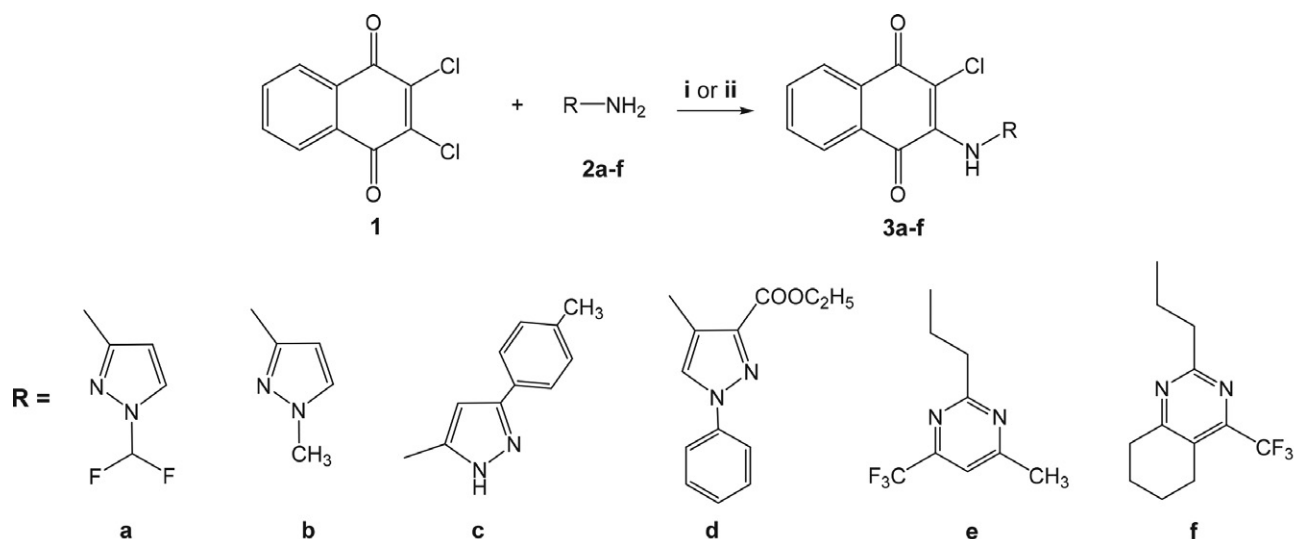
Scheme 1. Synthesis of aminopyrazole- ( 3a-d ) and aminopyrimidine ( 3e-f ) derivatives of dichloronaphthoquinone. Reagents and conditions: i EtOH/Na 2 CO 3 , reflux, 2 h; ii DMF/K 2 CO 3 , 65 °C, 4 h
