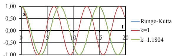
Fig. 1. The dimensionless x coordinates of the pendulum position as a function of the dimensionless time t obtained on the basis of various methods for solving non-linear dimensionless equation (21)
