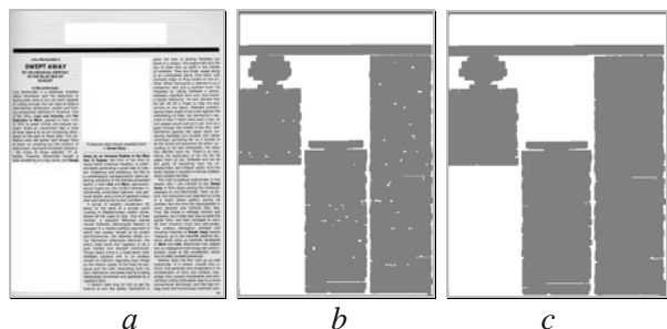
Fig. 5. The result of the extraction of text regions on the image of the scanned document: a – the original image; b – result after low-pass filtering and thresholding; c – the result of the filtering of connected components
