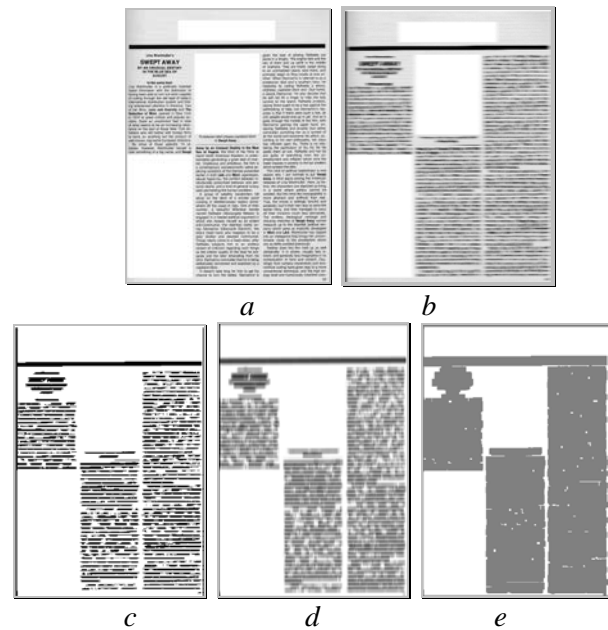
Fig. 2. Extraction of text regions on the image of the scanned document:
