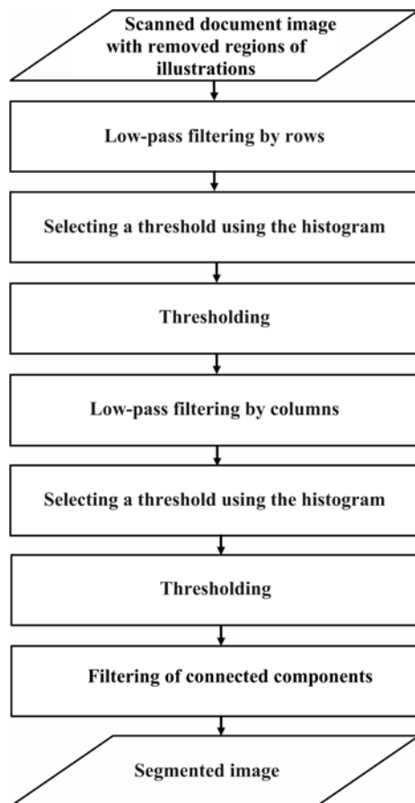
Fig. 1. The scheme of extraction of text regions of the scanned document image
