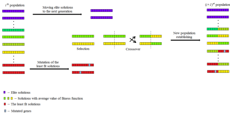
Figure 3: Scheme of the new population establishment for the modified genetic algorithm
