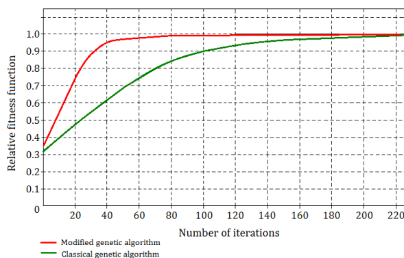
Figure 5: Objective function value dependence on the number of iterations during the process of optimization for the modified and the classical genetic algorithm
