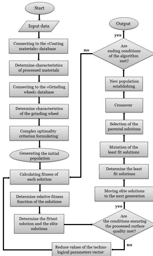
Figure 4: Modified genetic algorithm for optimization of plasma coatings grinding process
