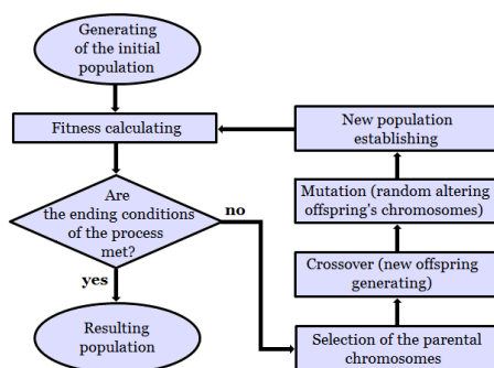
Figure 1: General scheme of the classical genetic algorithm
