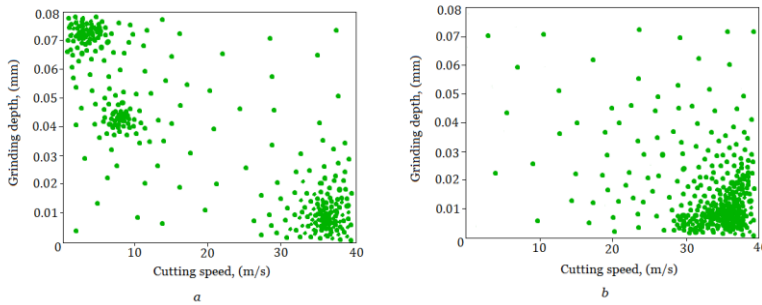
Figure 2: Distribution of chromosomes for the classical genetic algorithm: a – grouping around several extremums; b – dominating of one of the extremums and driving out other solutions from the population
