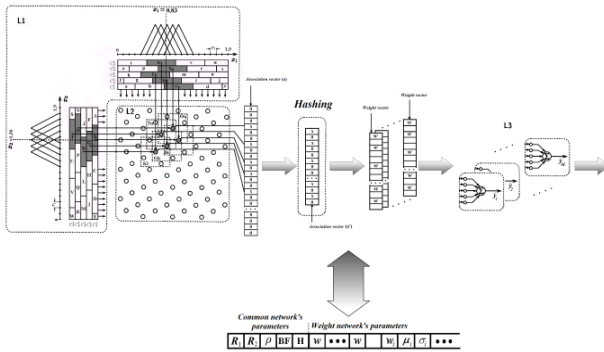
Fig. 1. Albus network
