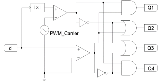
Fig. 3. PWM circuitry.
