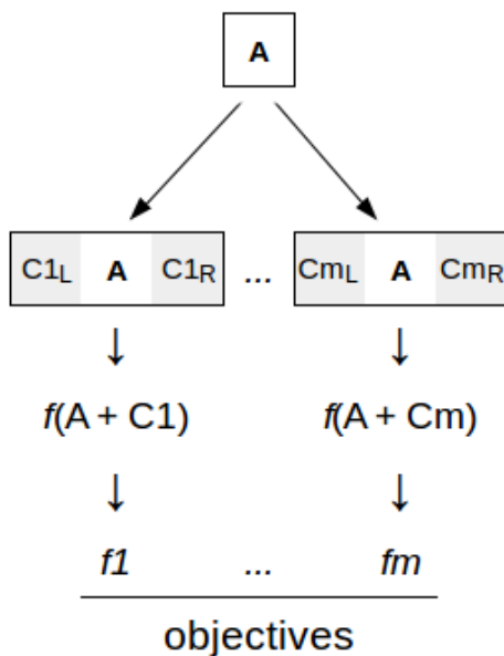
Figure 4. Fitness evaluations f1,..., fm of A in contextes C1,..., Cm
