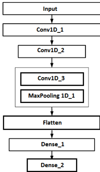
Fig. 4. 1D CNN general architecture for sale prediction
