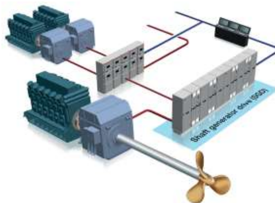
Fig. 1. Configuration of a typical Ship's Energy System with Shaft Generator Drive [2]
