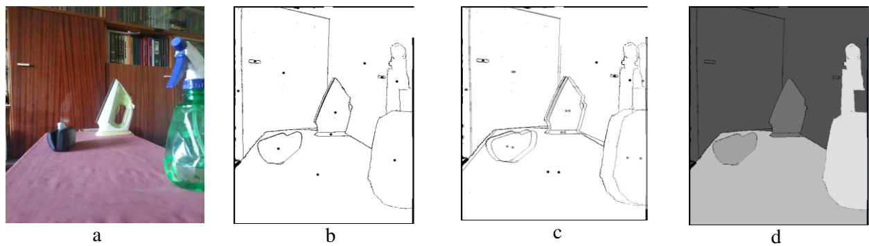
Fig. 4. Modeling the proposed method: a – scene image; b – contour description of the one of stereopair image; c – stereopair images contour combination and mass centers evaluation; d – depth map coloring
