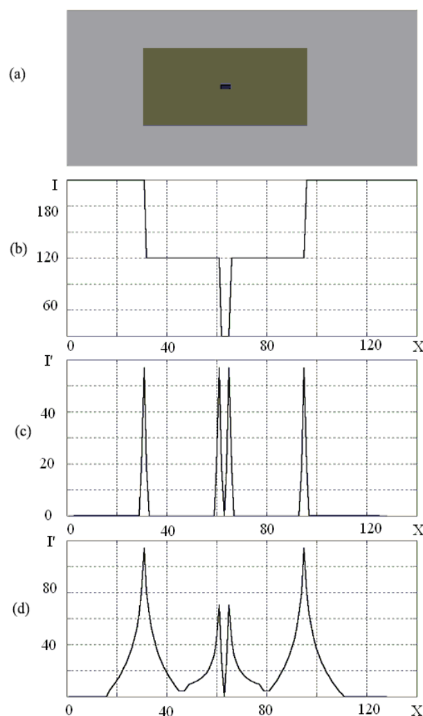
Fig. 1. Modeling results: (a), (b) – test image and its line; (c), (d) – image line in the wavelet transform domain for Gauss Wavelet Transform on different scales s_2 > s_1 Source: compiled by [15]
