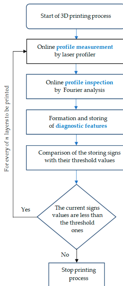
Figure 10. Monitoring algorithm block diagram.
